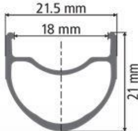
RR421 rim dimensions- disc asym
