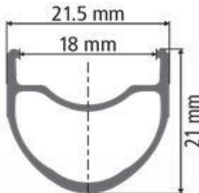
RR411 rim dimensions- rim brake
