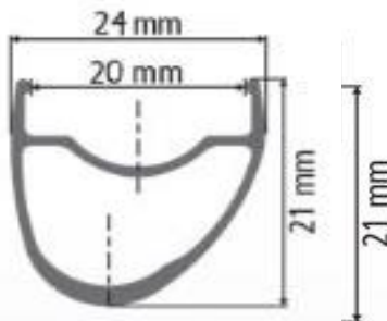
RR421 rim dimensions- disc asym
