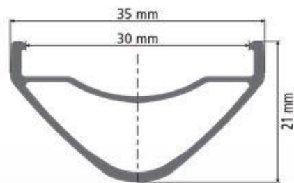
XM481 rim dimensions- wide option
