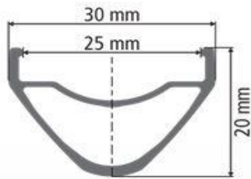
XM421 rim dimensions
