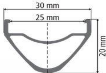
XM421 rim dimensions
